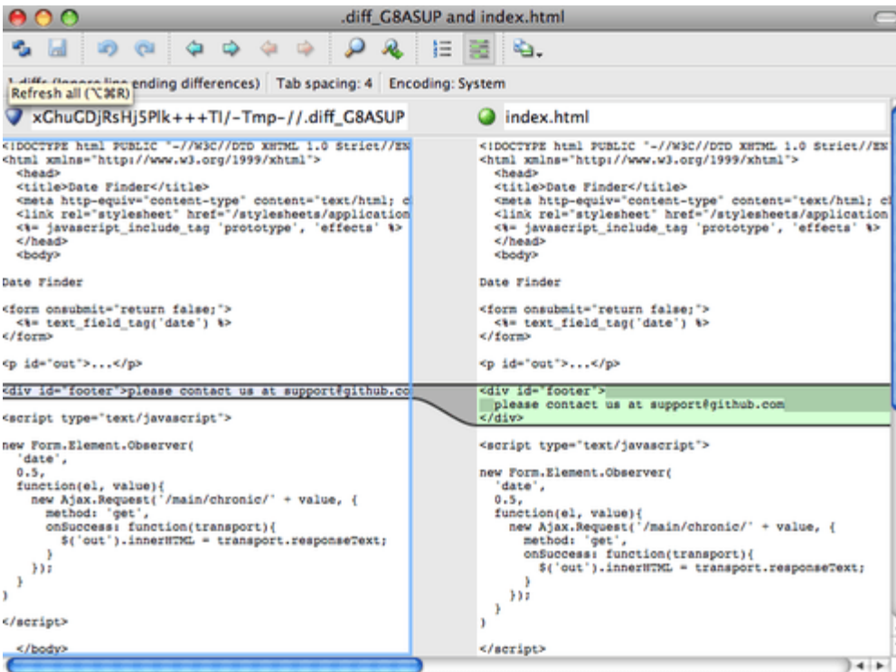
Figure 143. P4Merge.
